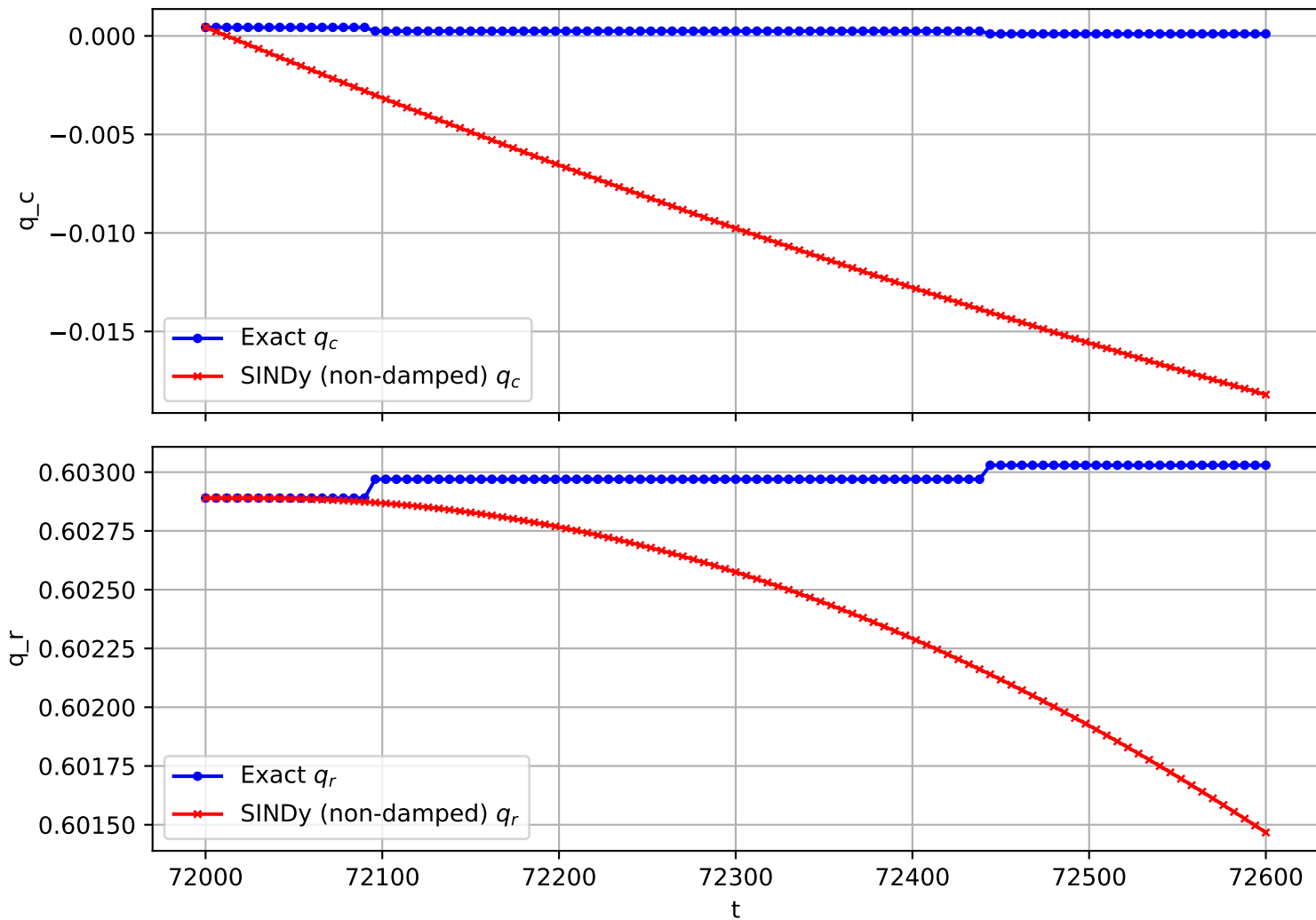
Trajectory 2846 (non-damped)
