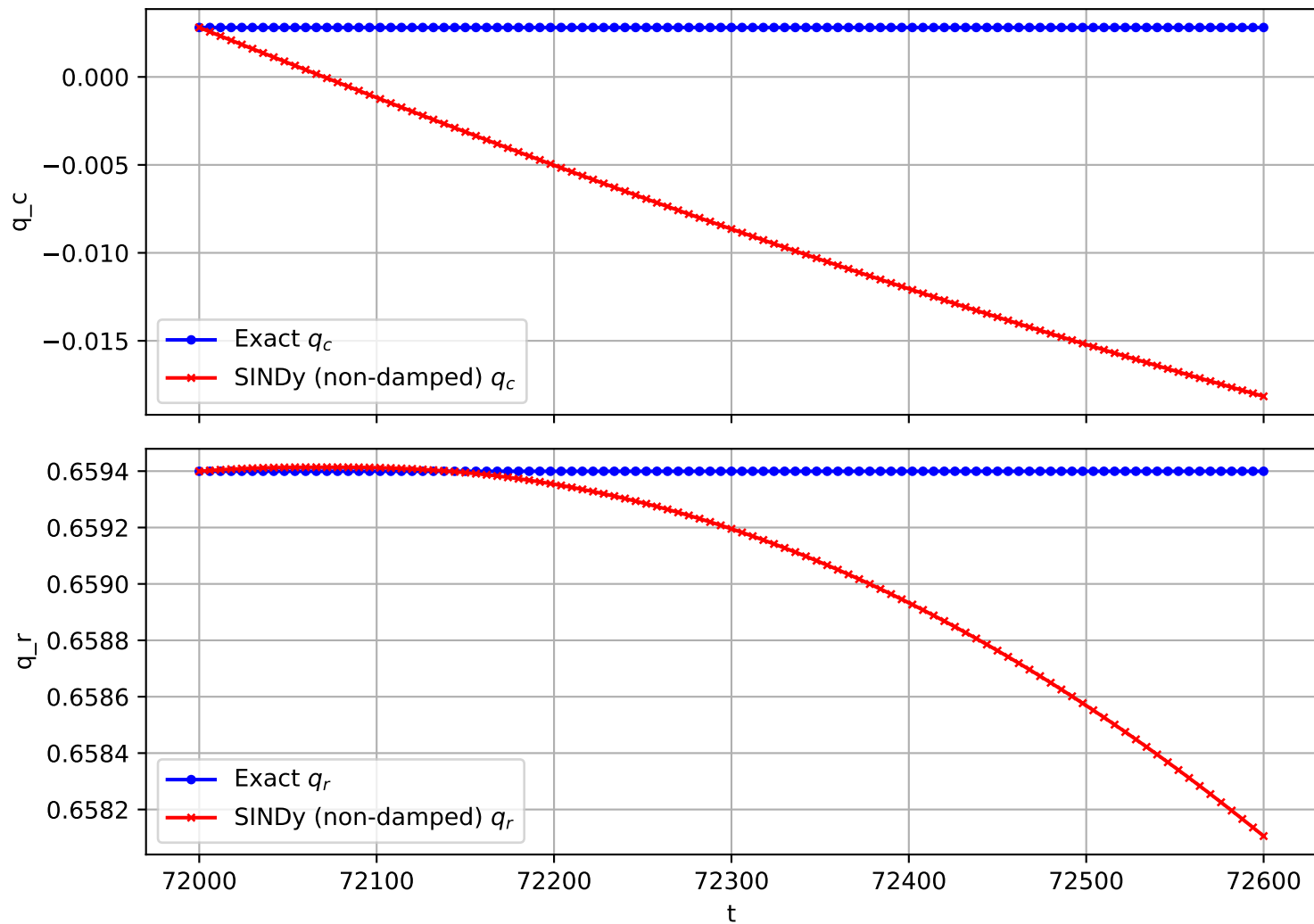
Trajectory 2849 (non-damped)
