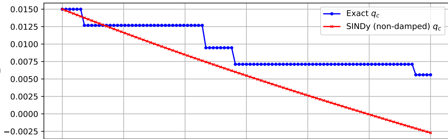
Trajectory 2853 (non-damped)
