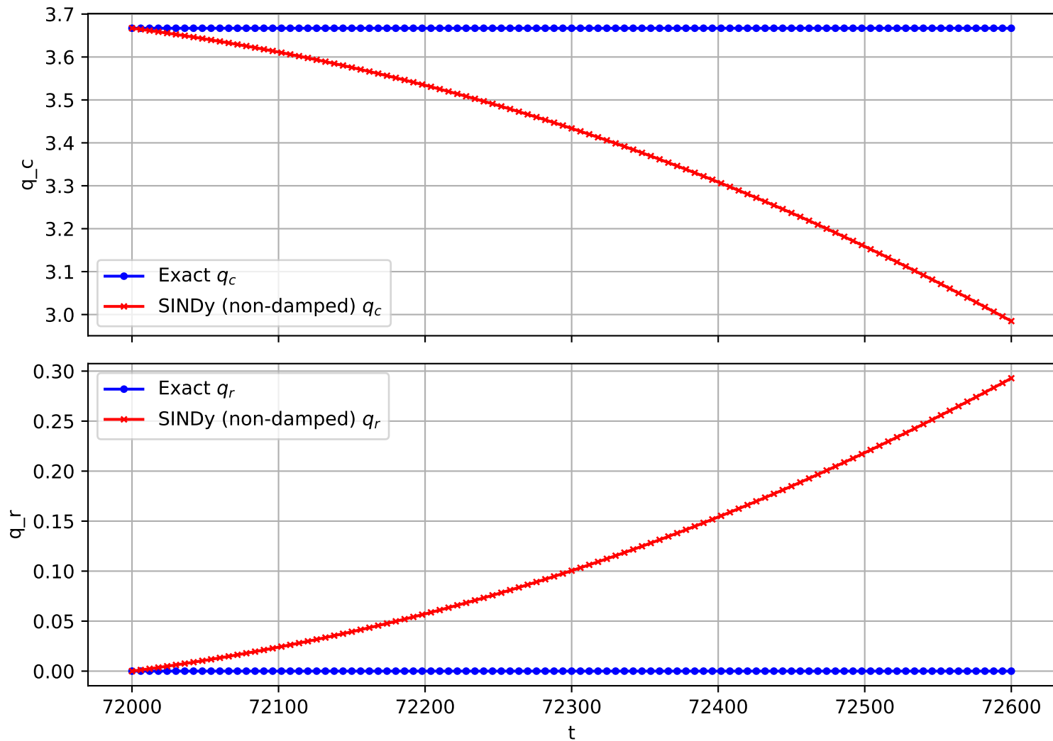
Trajectory 2858 (non-damped)
