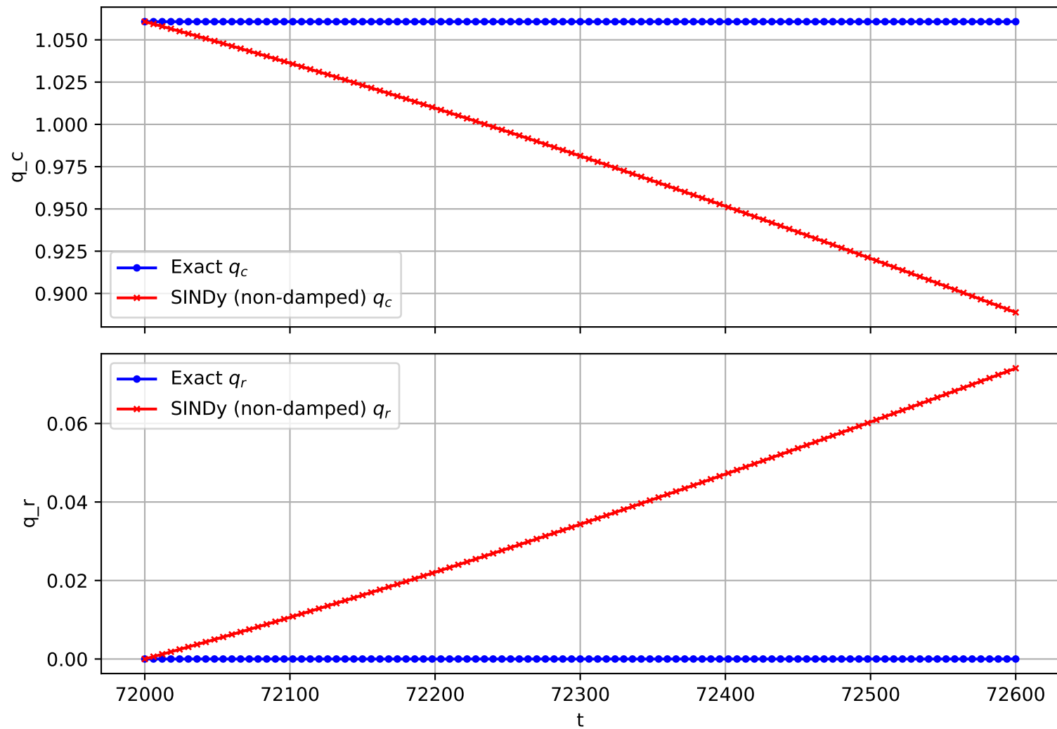
Trajectory 2859 (non-damped)
