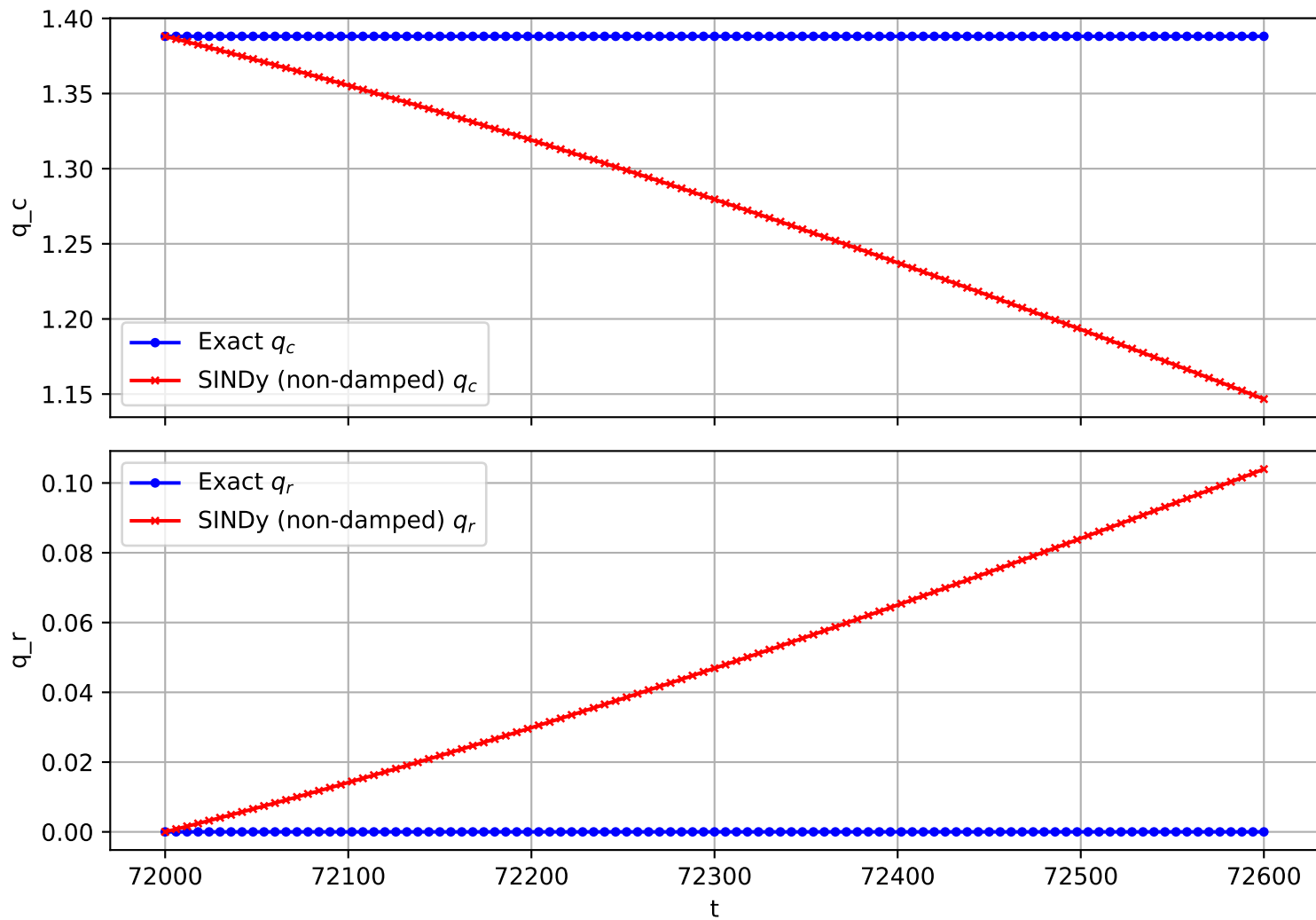
Trajectory 2863 (non-damped)
