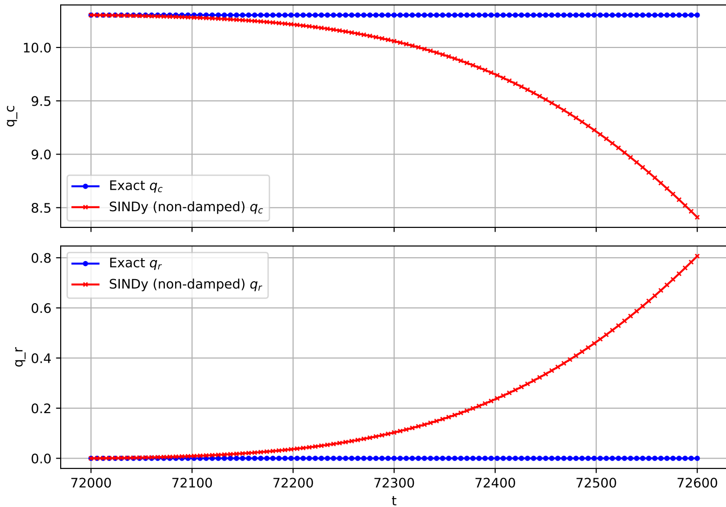
Trajectory 2870 (non-damped)
