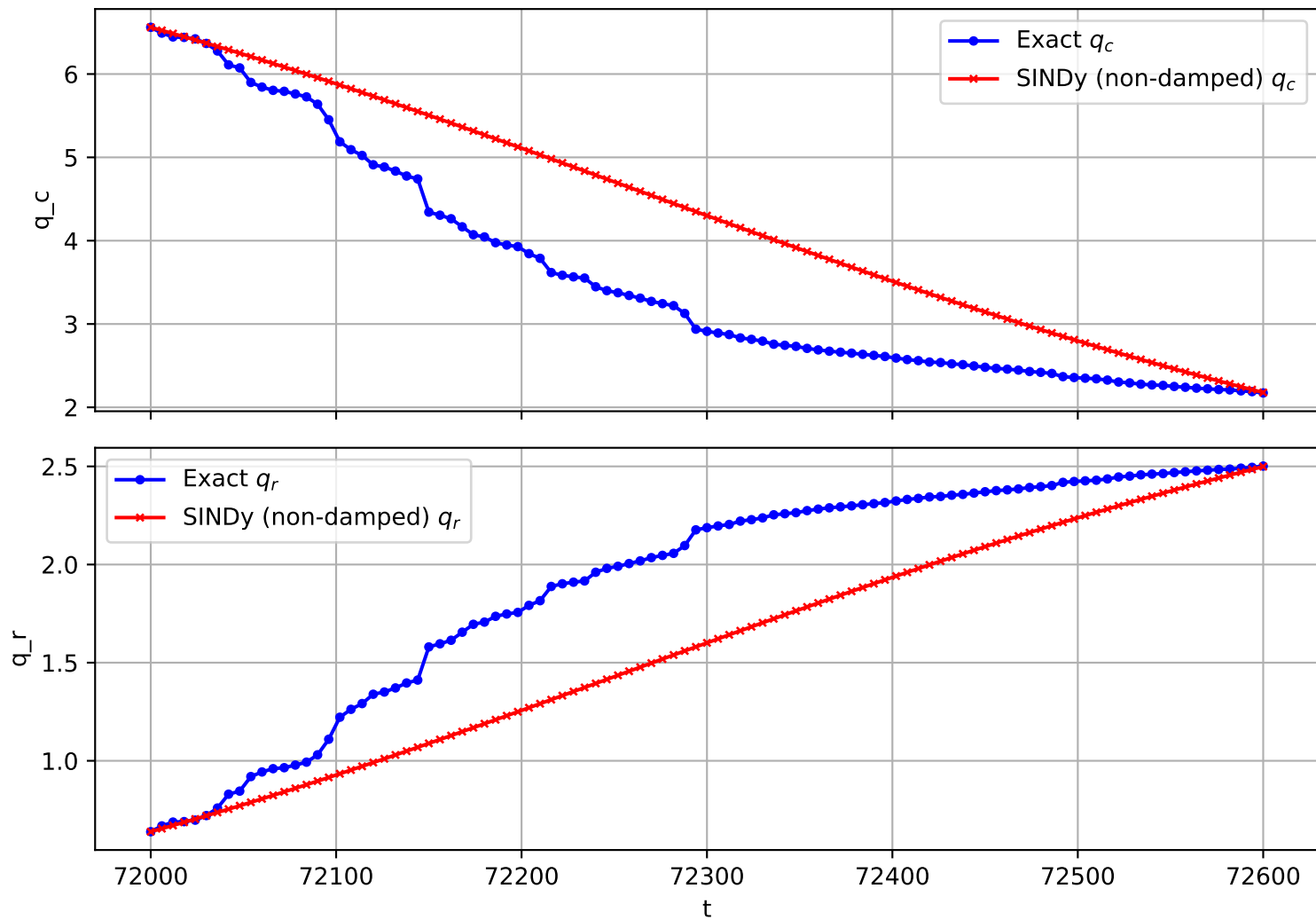
Trajectory 2876 (non-damped)
