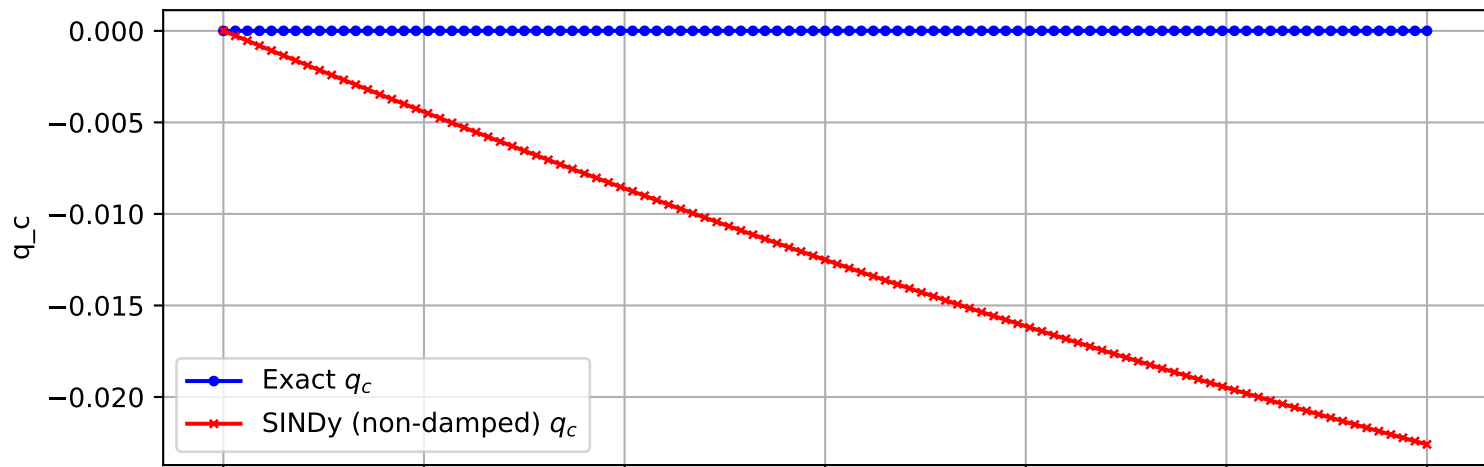
Trajectory 2882 (non-damped)
