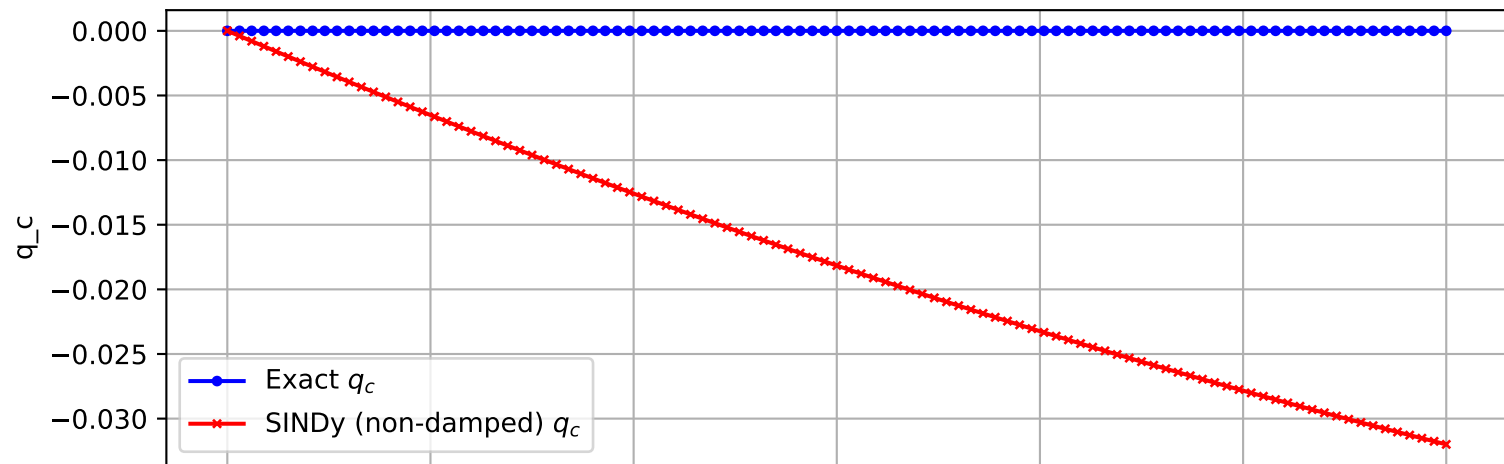
Trajectory 2886 (non-damped)
