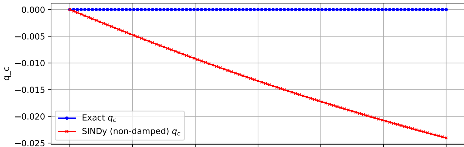
Trajectory 2887 (non-damped)
