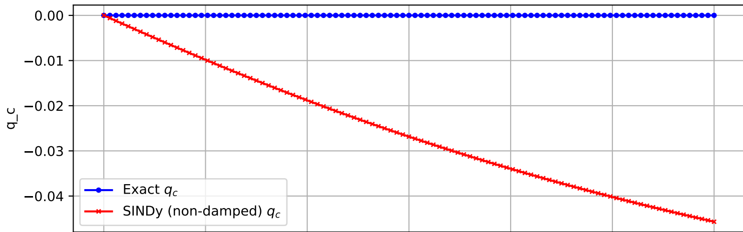
Trajectory 2888 (non-damped)
