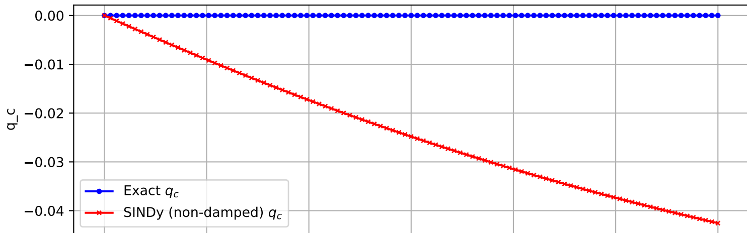
Trajectory 2889 (non-damped)
