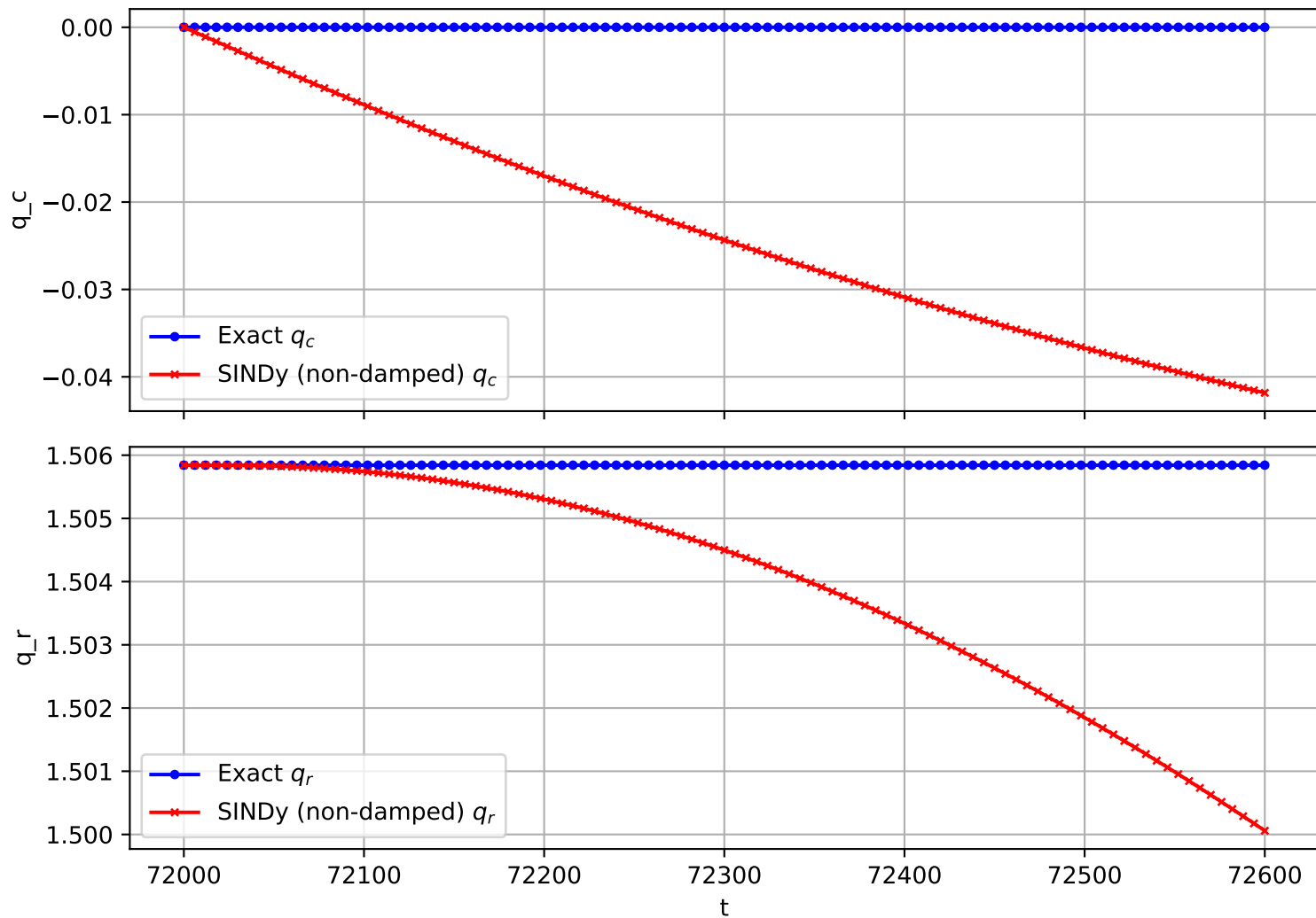
Trajectory 289 (non-damped)
