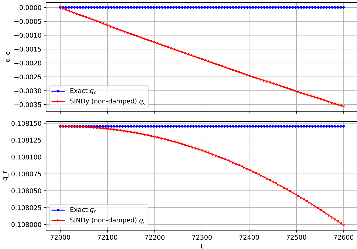
Trajectory 2895 (non-damped)
