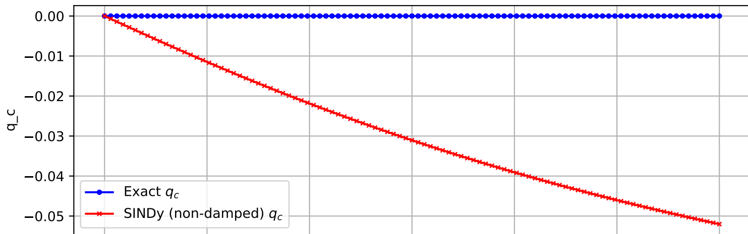
Trajectory 290 (non-damped)
