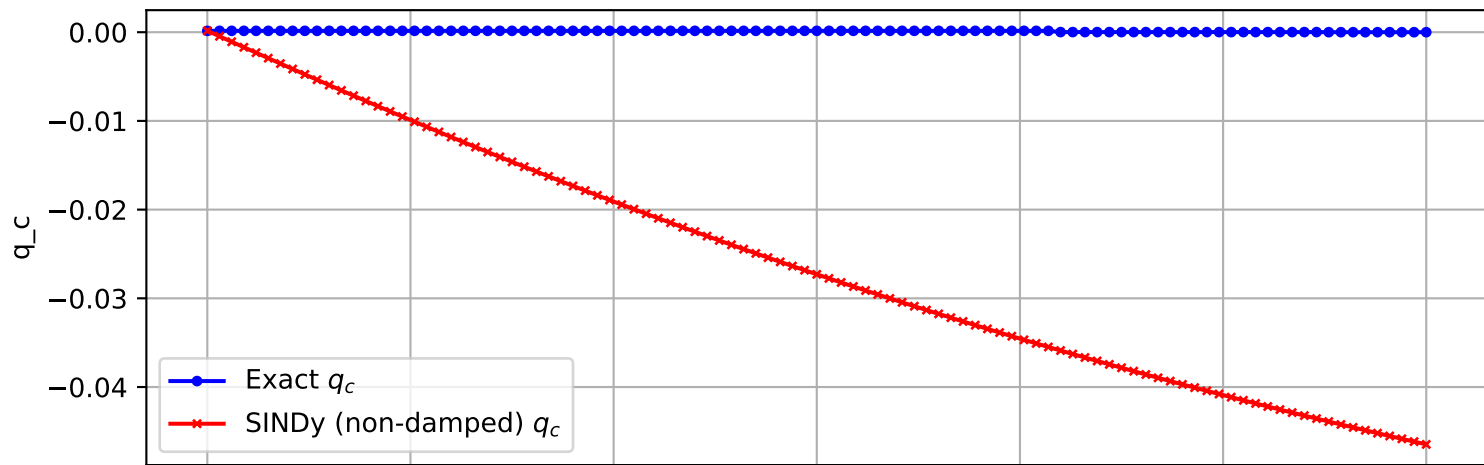
Trajectory 2906 (non-damped)
