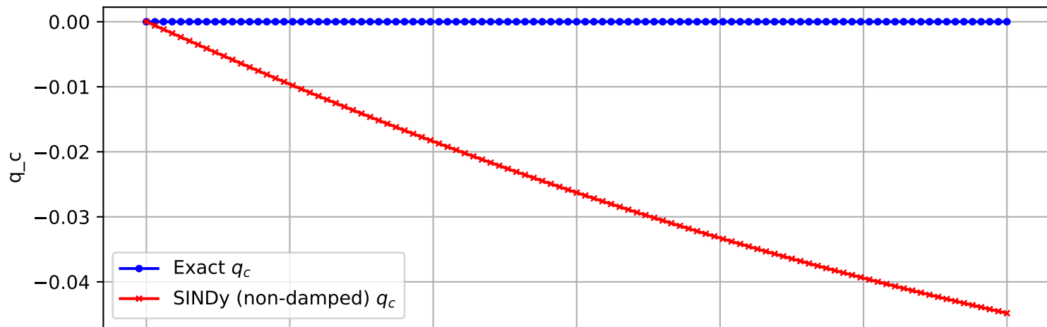
Trajectory 2907 (non-damped)
