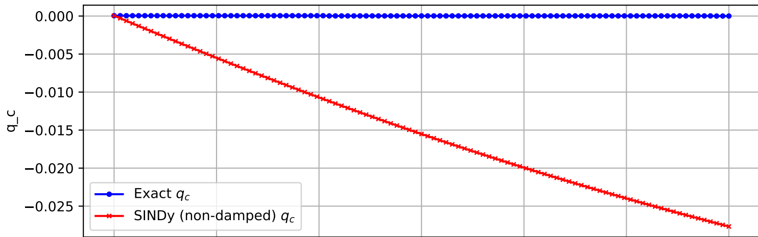
Trajectory 2909 (non-damped)
