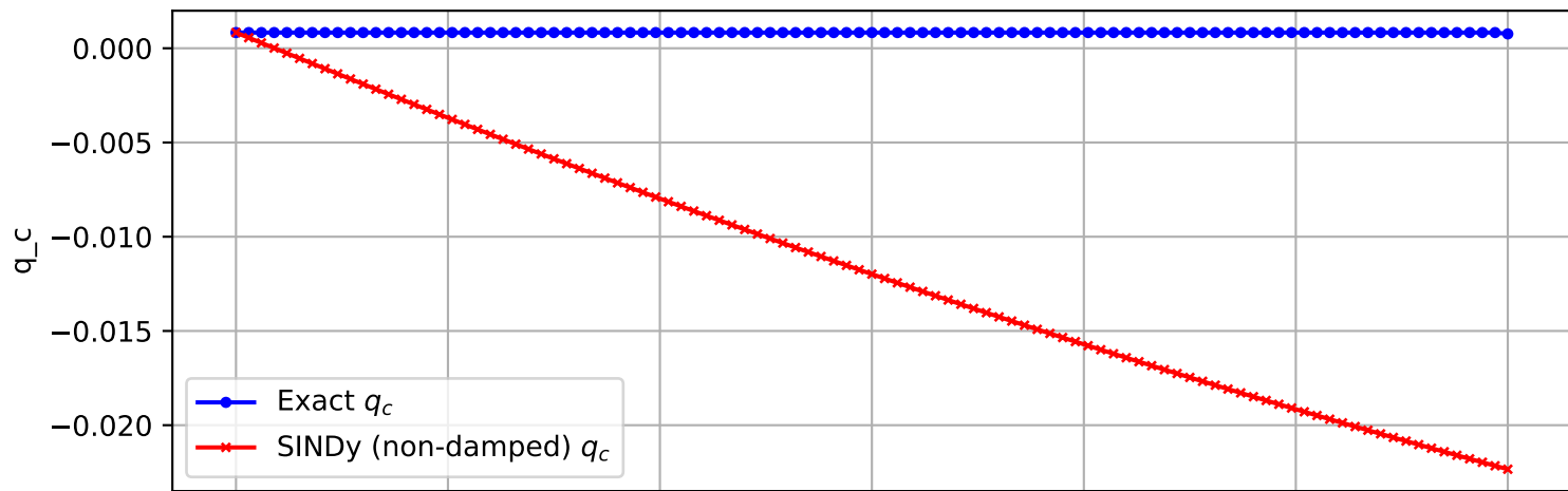
Trajectory 2910 (non-damped)
