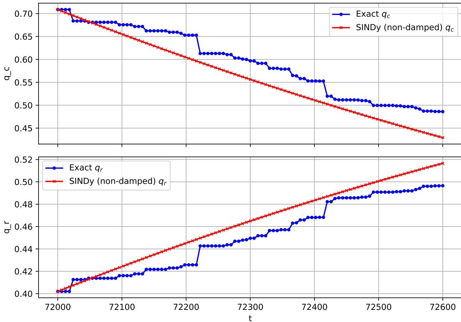
Trajectory 2917 (non-damped)
