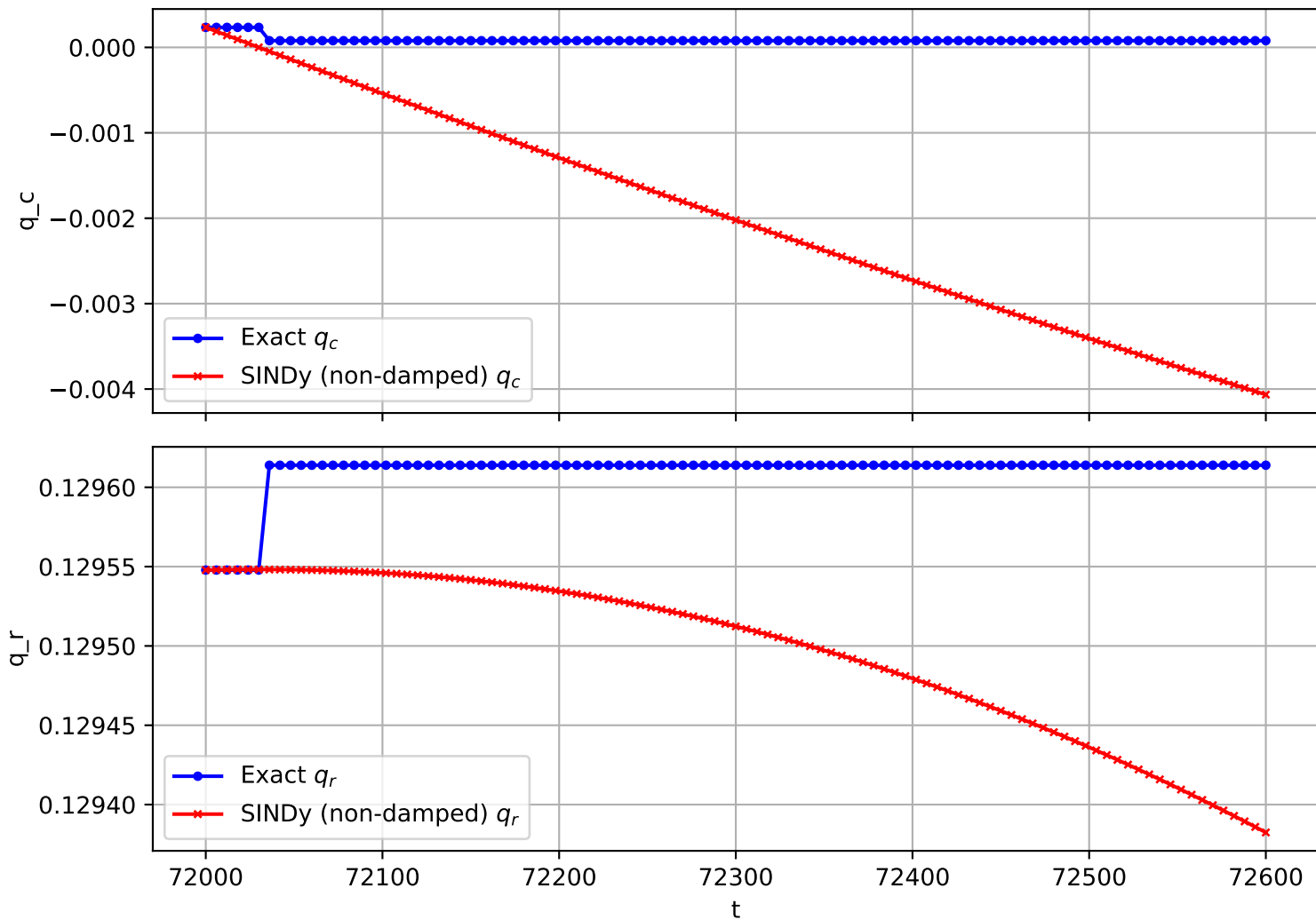
Trajectory 2920 (non-damped)
