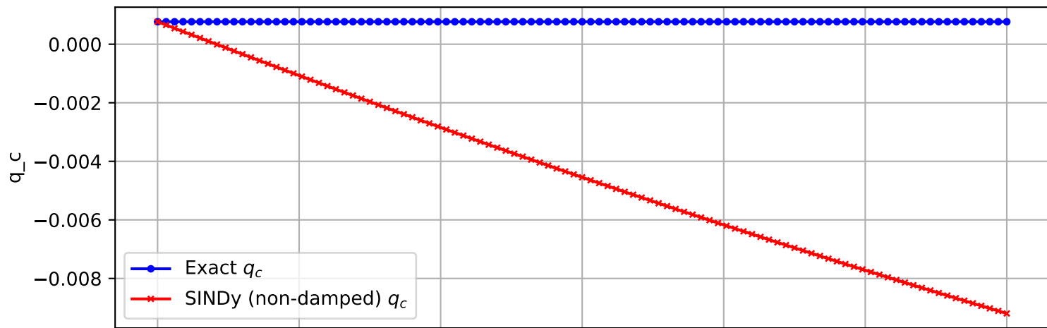
Trajectory 2925 (non-damped)
