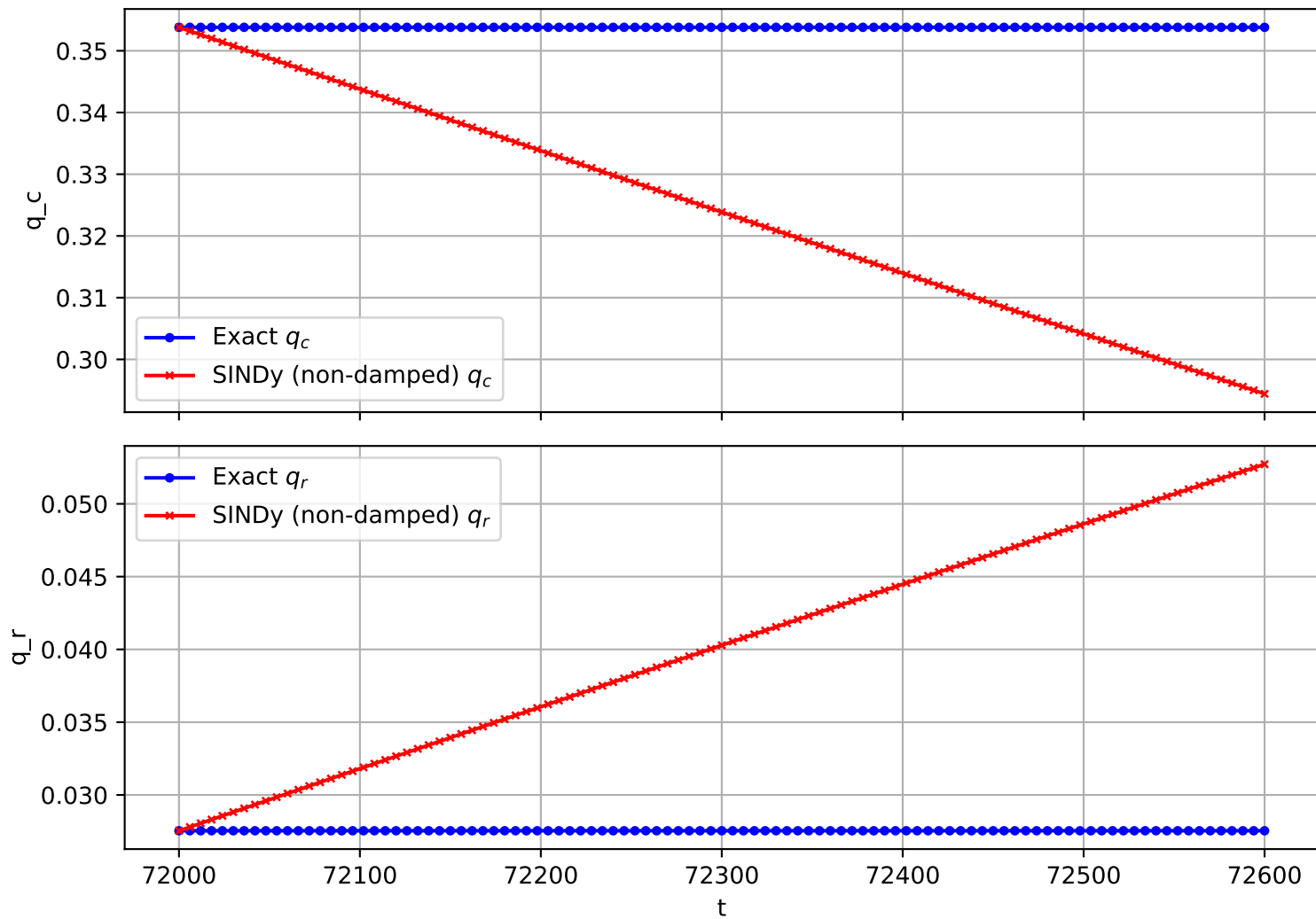
Trajectory 2931 (non-damped)
