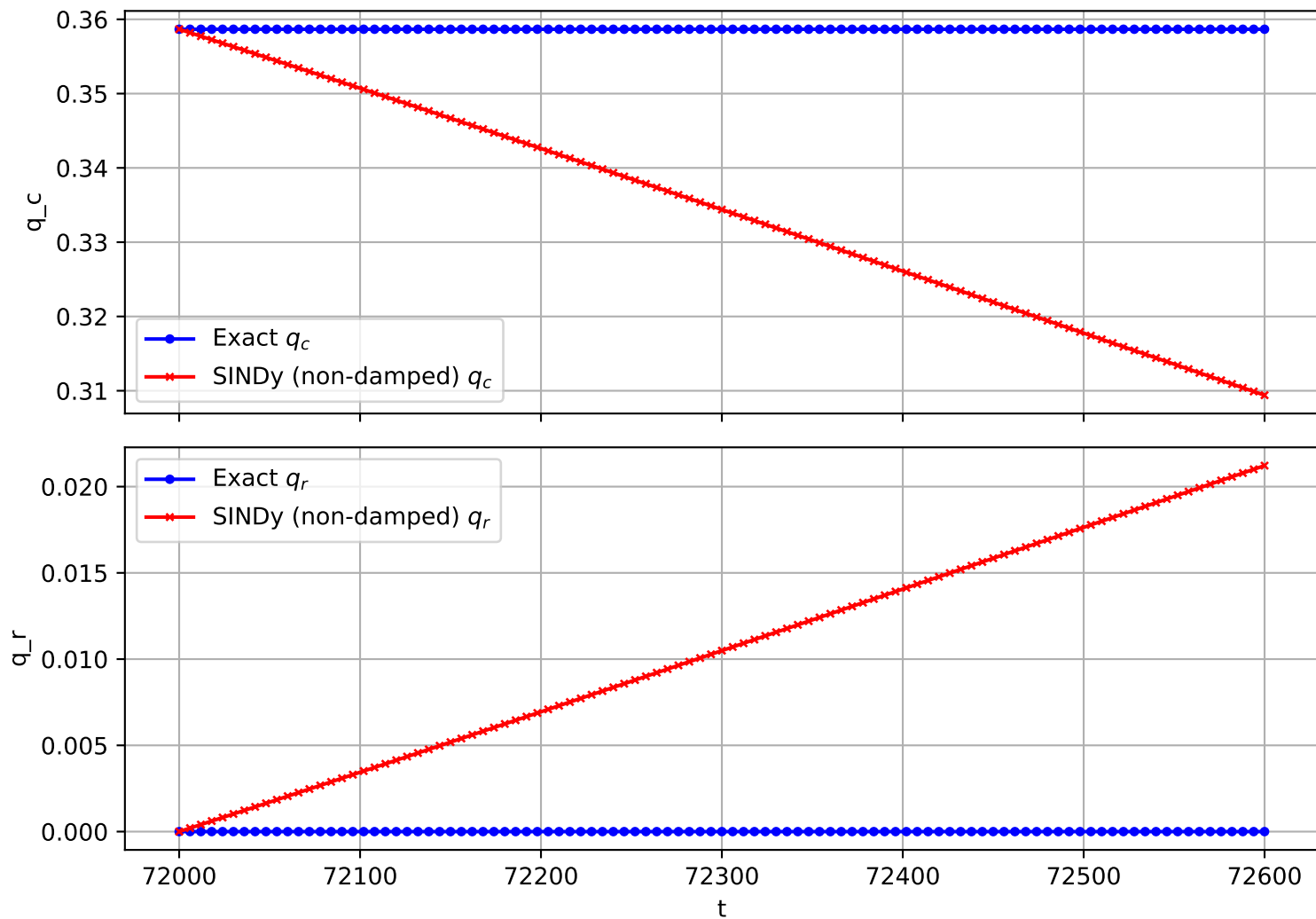
Trajectory 2934 (non-damped)
