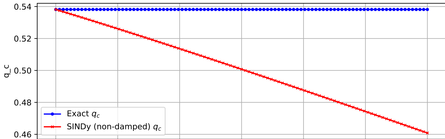
Trajectory 2944 (non-damped)
