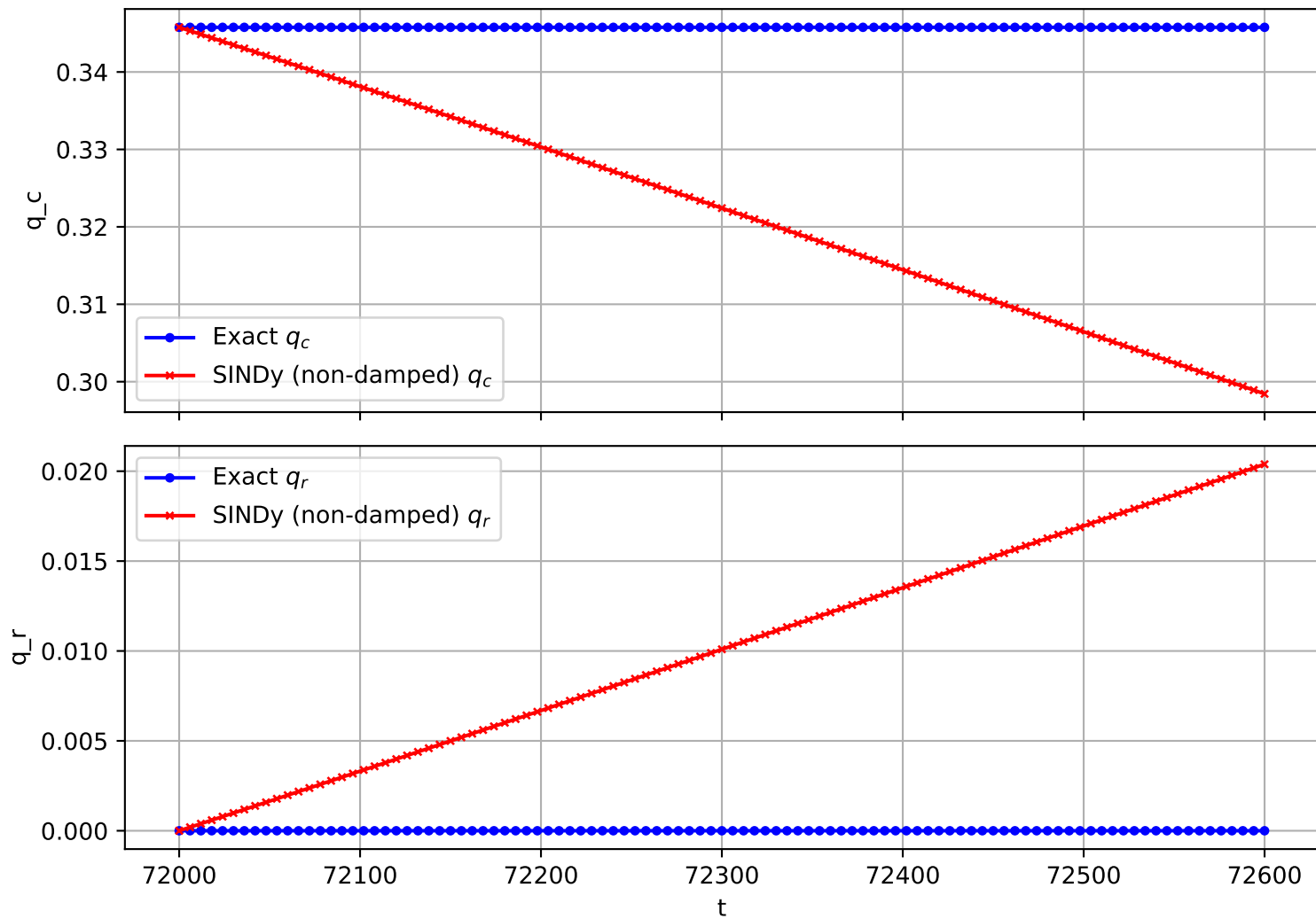
Trajectory 2953 (non-damped)
