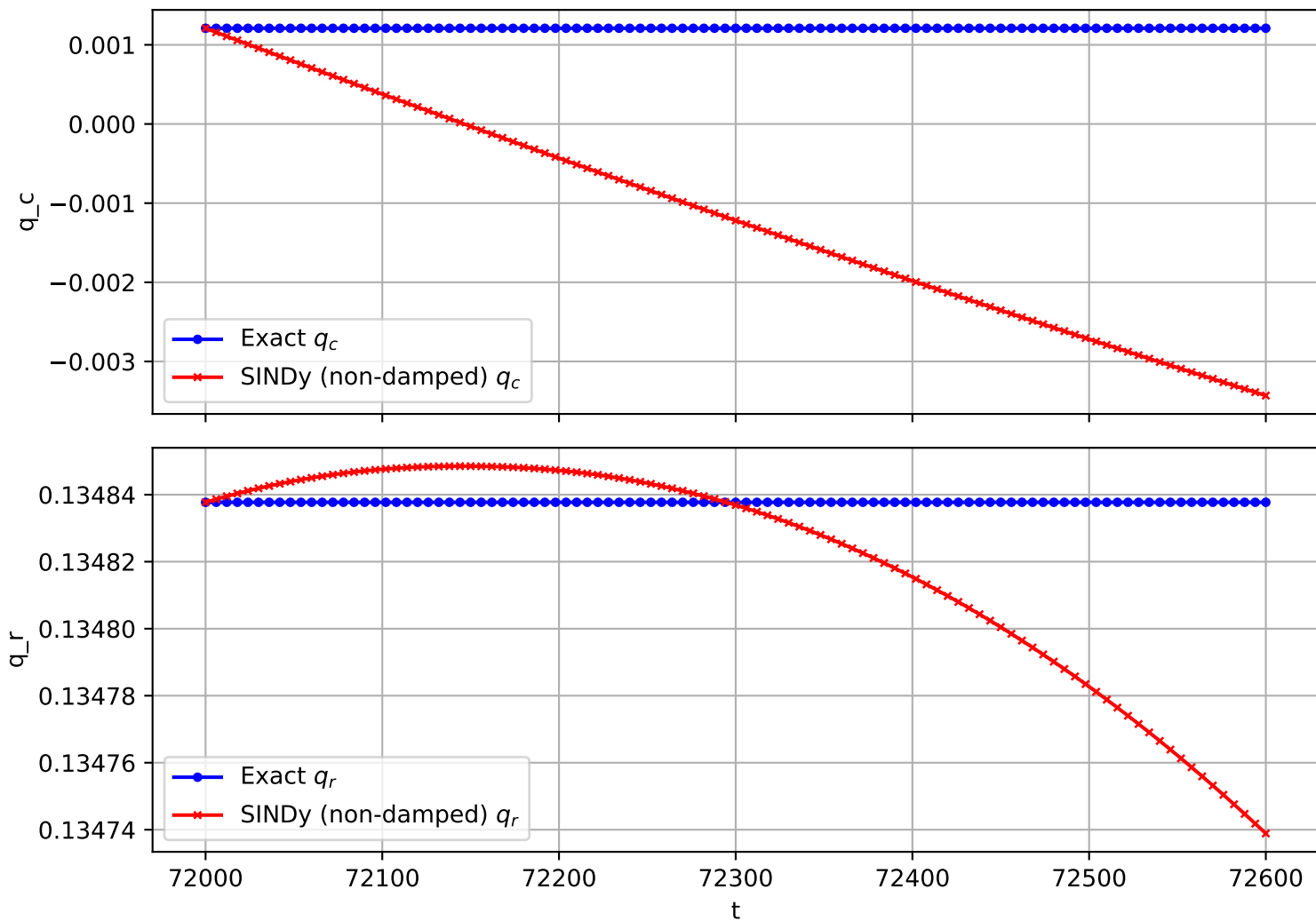
Trajectory 2963 (non-damped)
