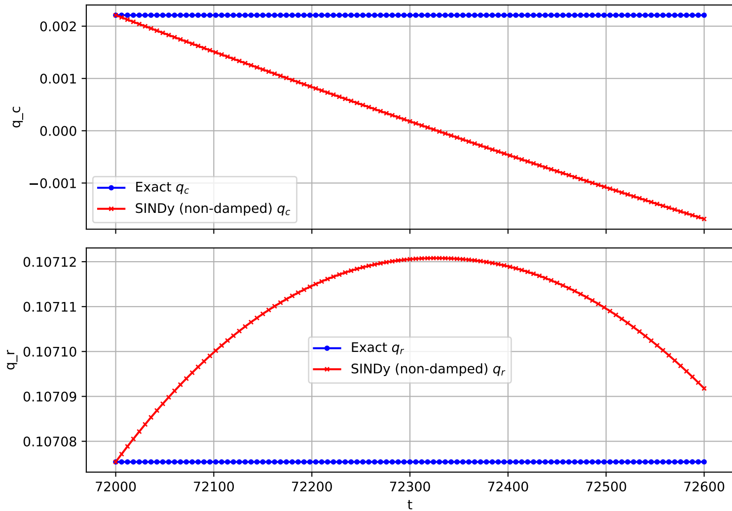
Trajectory 2964 (non-damped)
