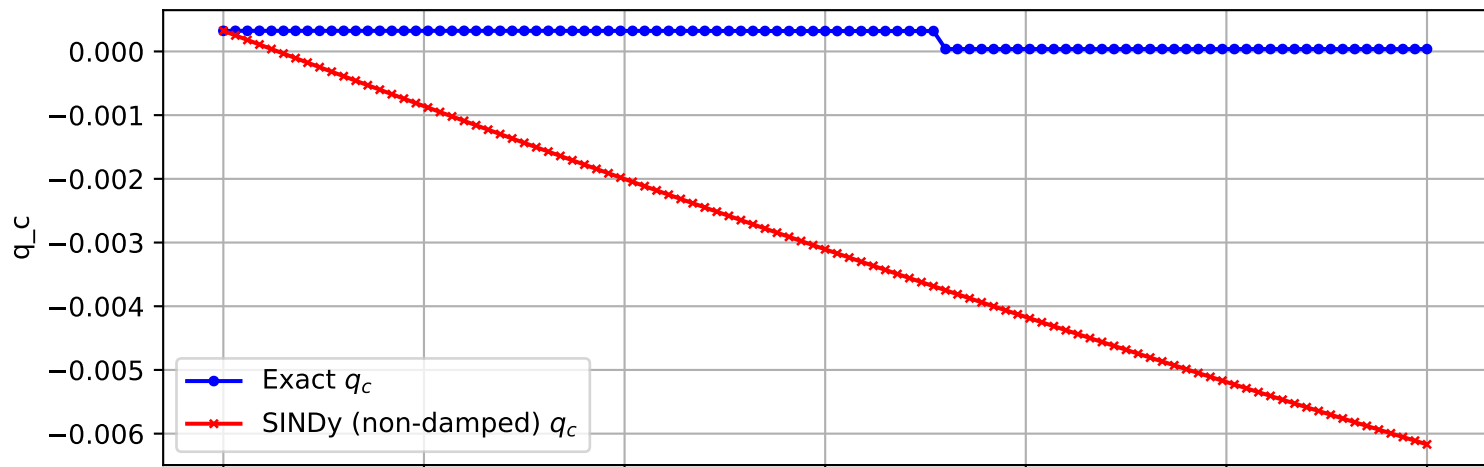
Trajectory 2965 (non-damped)
