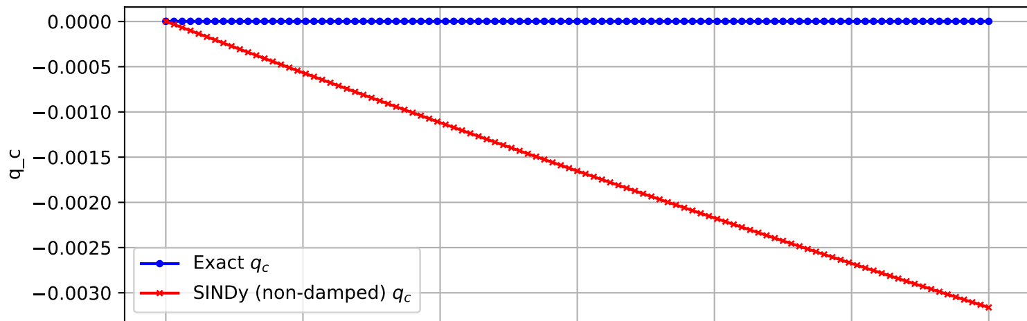
Trajectory 2970 (non-damped)
