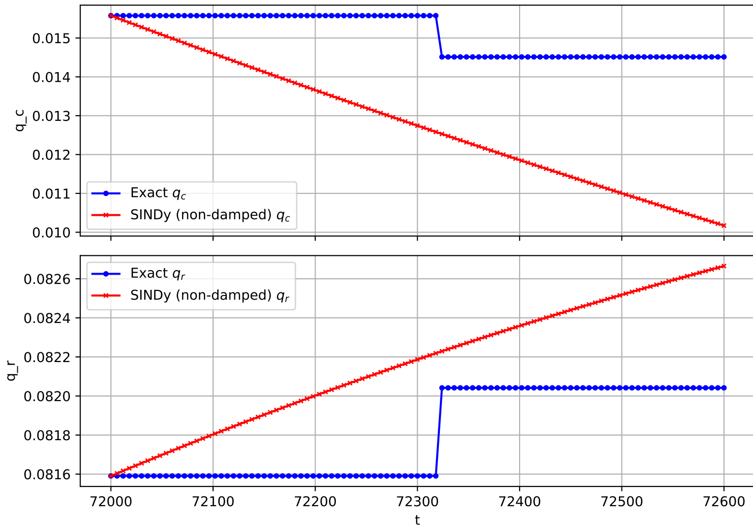
Trajectory 2976 (non-damped)
