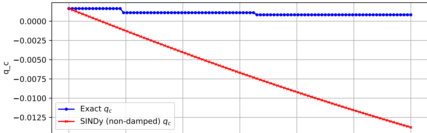
Trajectory 2979 (non-damped)
