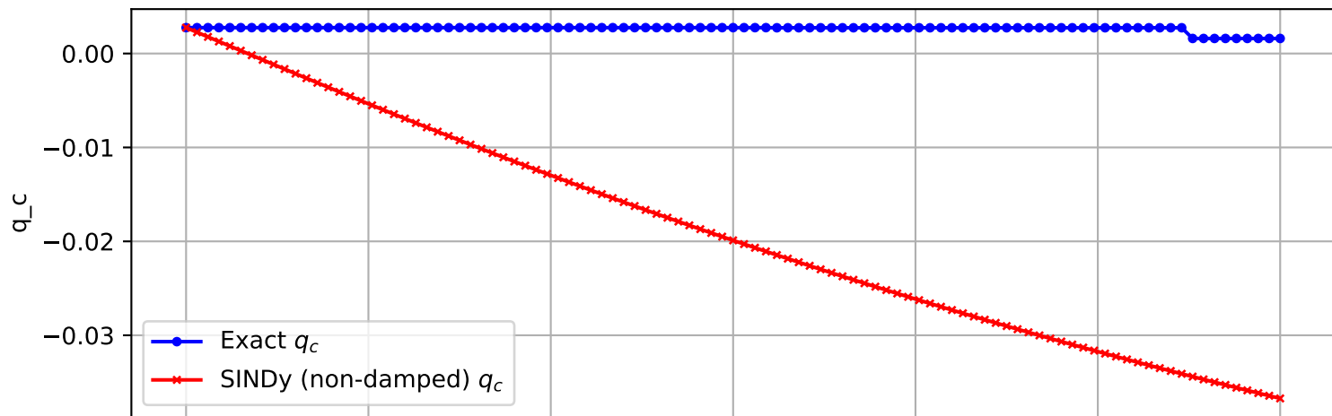
Trajectory 2983 (non-damped)
