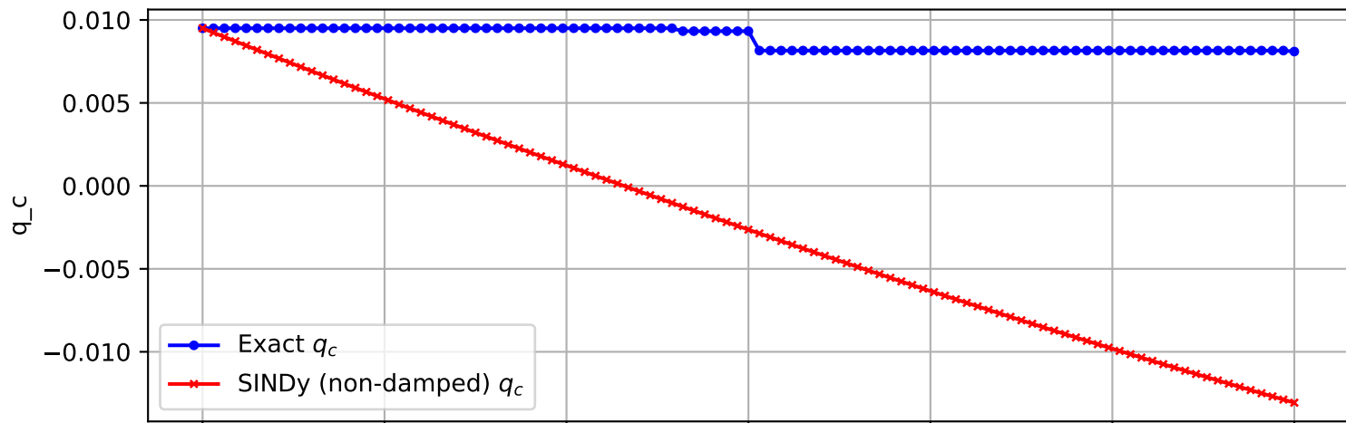
Trajectory 2987 (non-damped)
