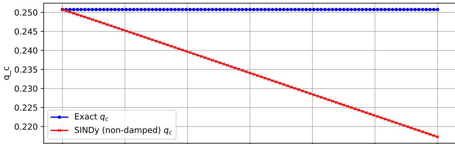
Trajectory 2999 (non-damped)
