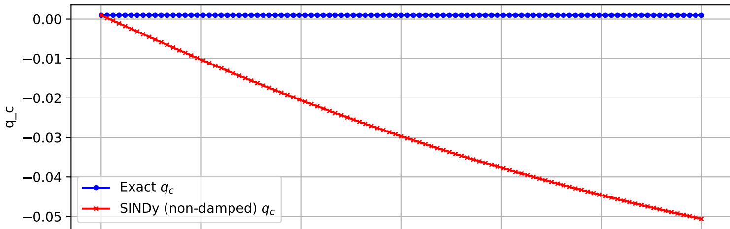
Trajectory 300 (non-damped)
