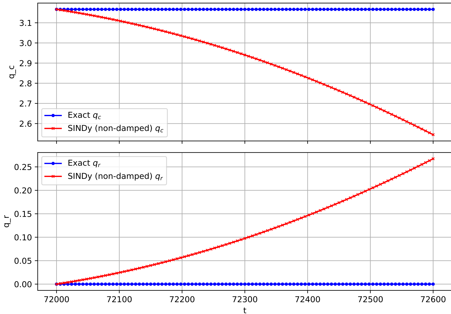
Trajectory 3004 (non-damped)
