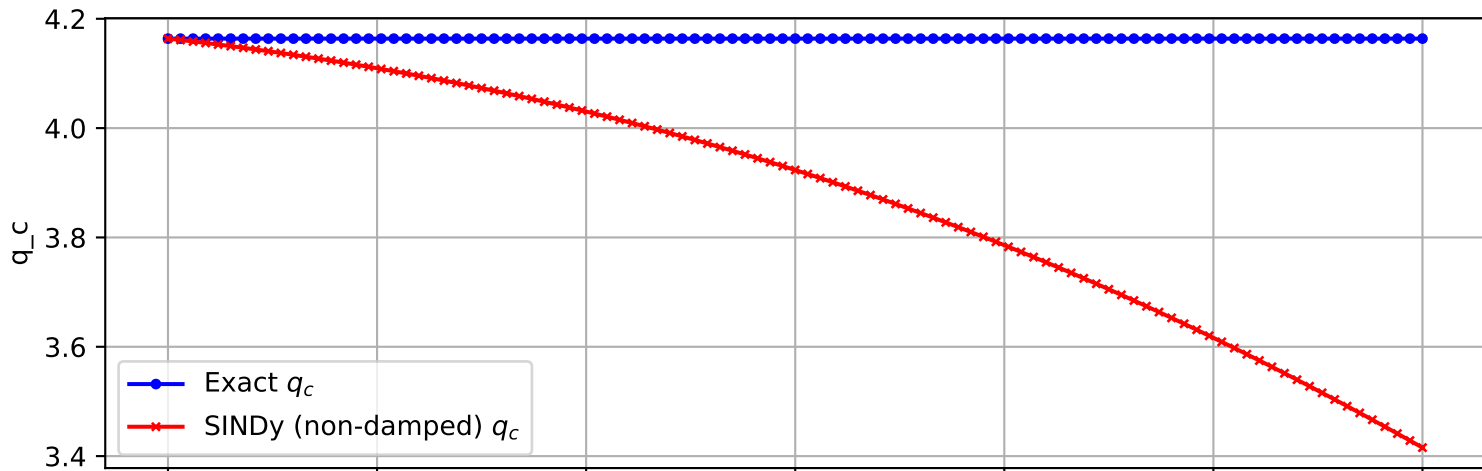
Trajectory 3009 (non-damped)
