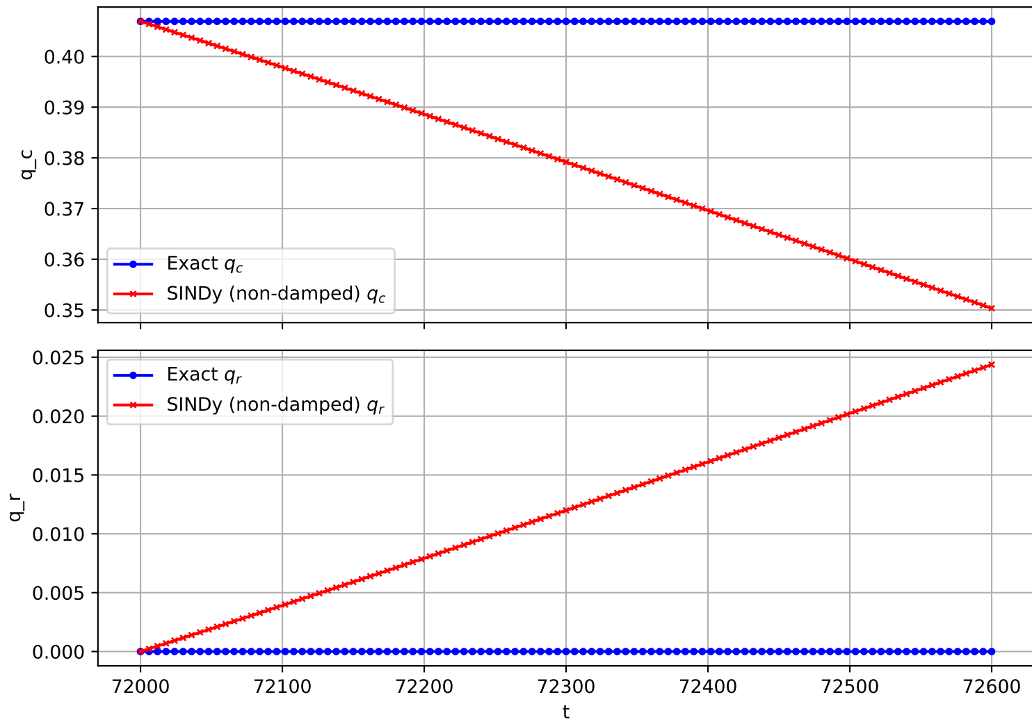
Trajectory 3011 (non-damped)
