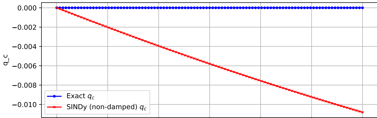
Trajectory 3013 (non-damped)
