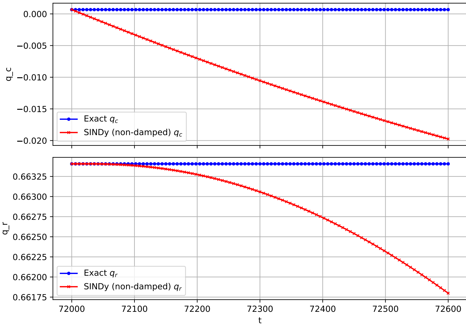
Trajectory 3014 (non-damped)
