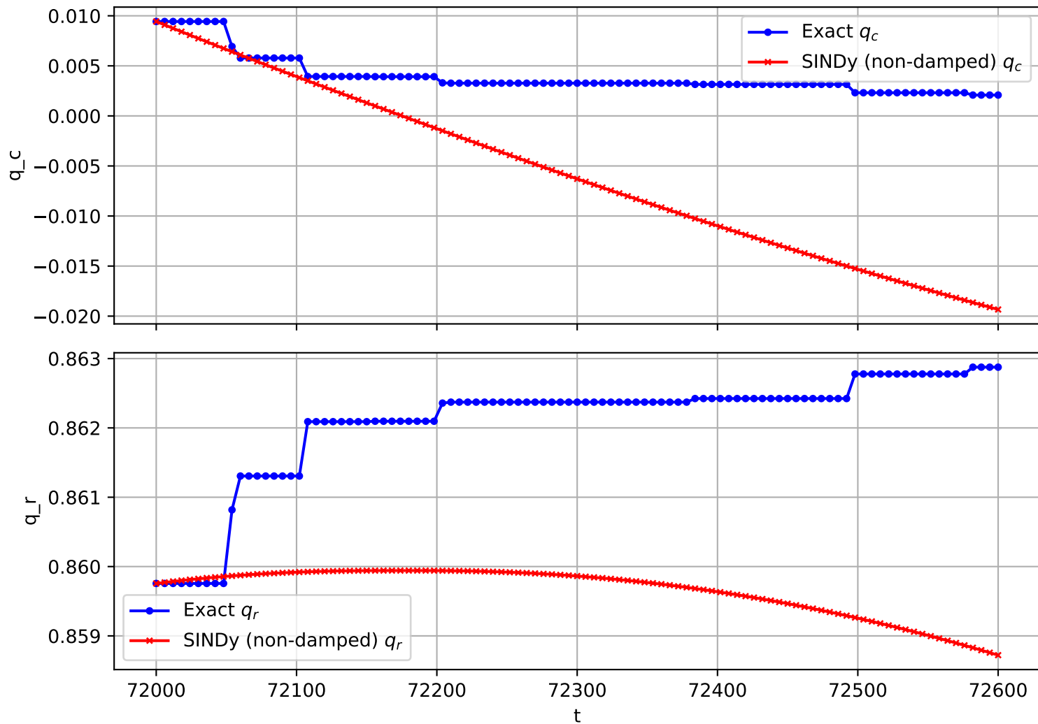
Trajectory 3016 (non-damped)
