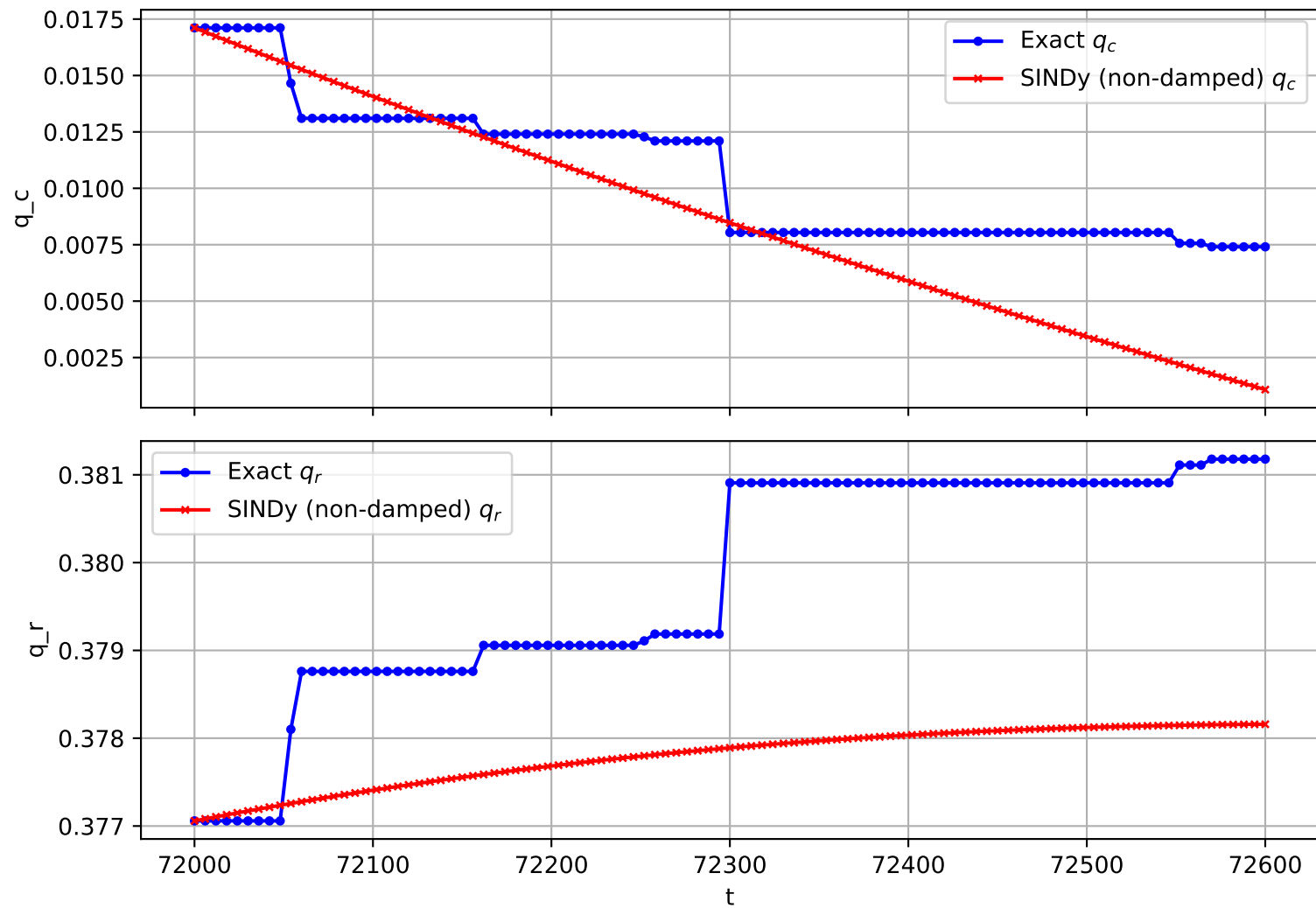
Trajectory 3018 (non-damped)
