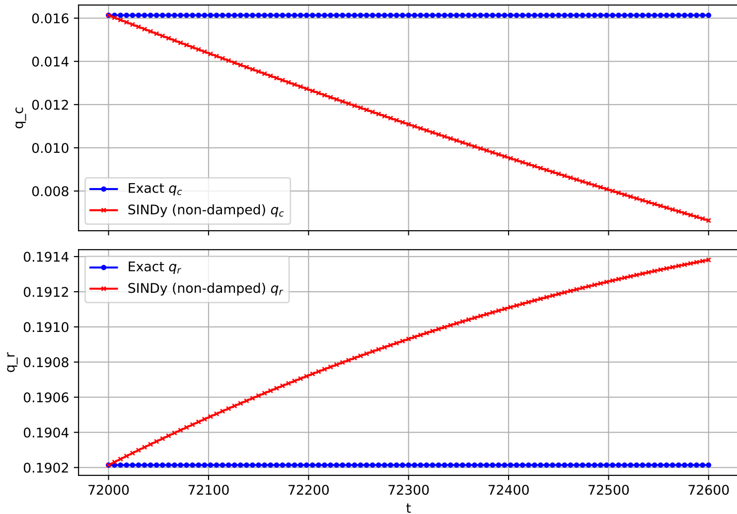
Trajectory 3019 (non-damped)
