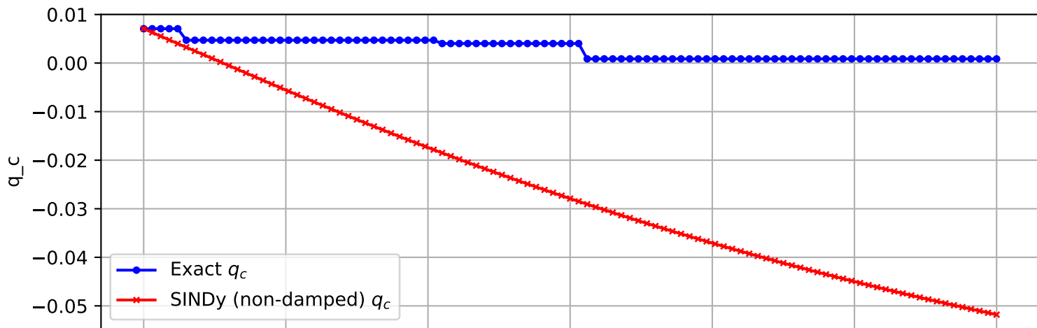
Trajectory 302 (non-damped)
