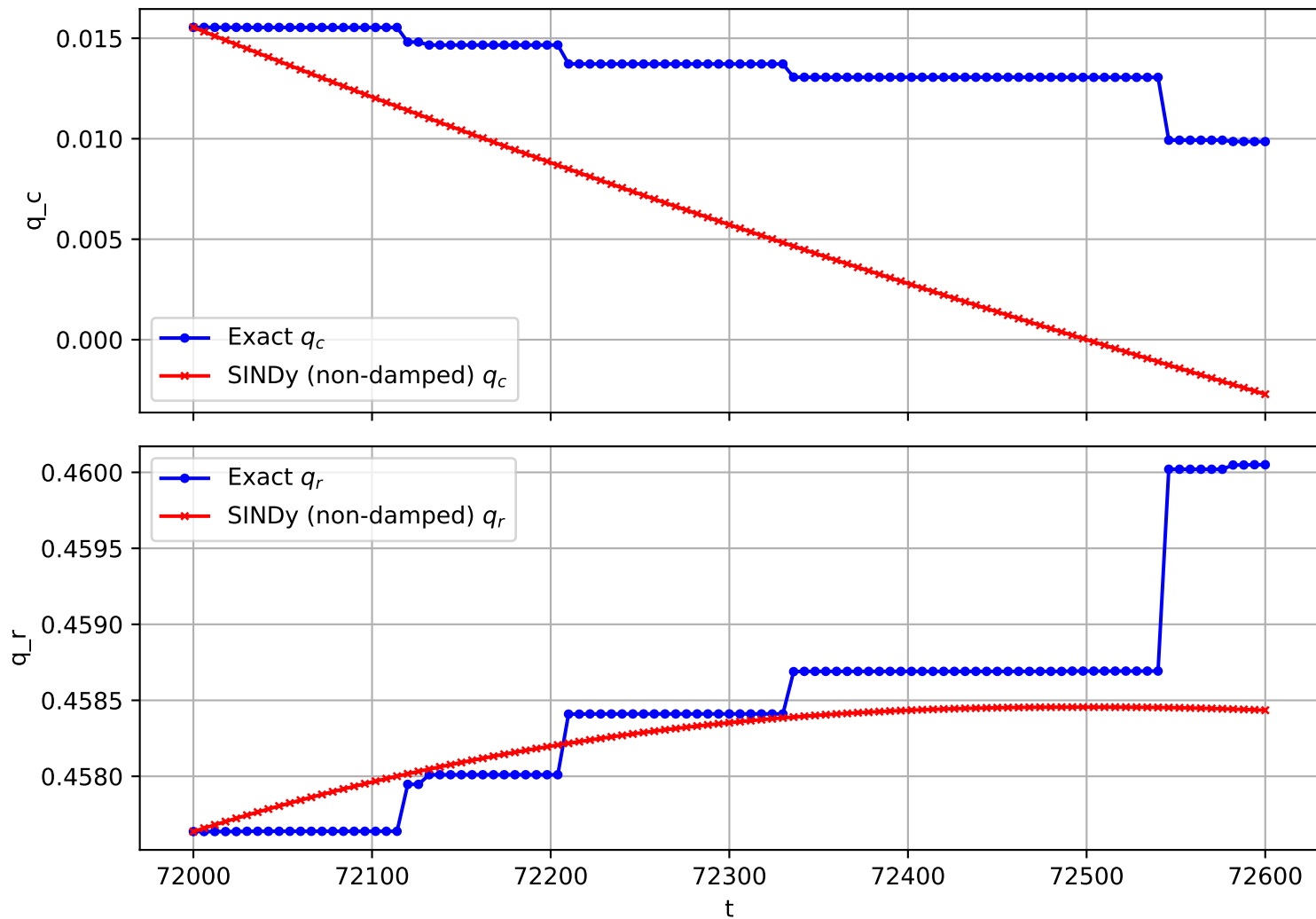
Trajectory 3021 (non-damped)
