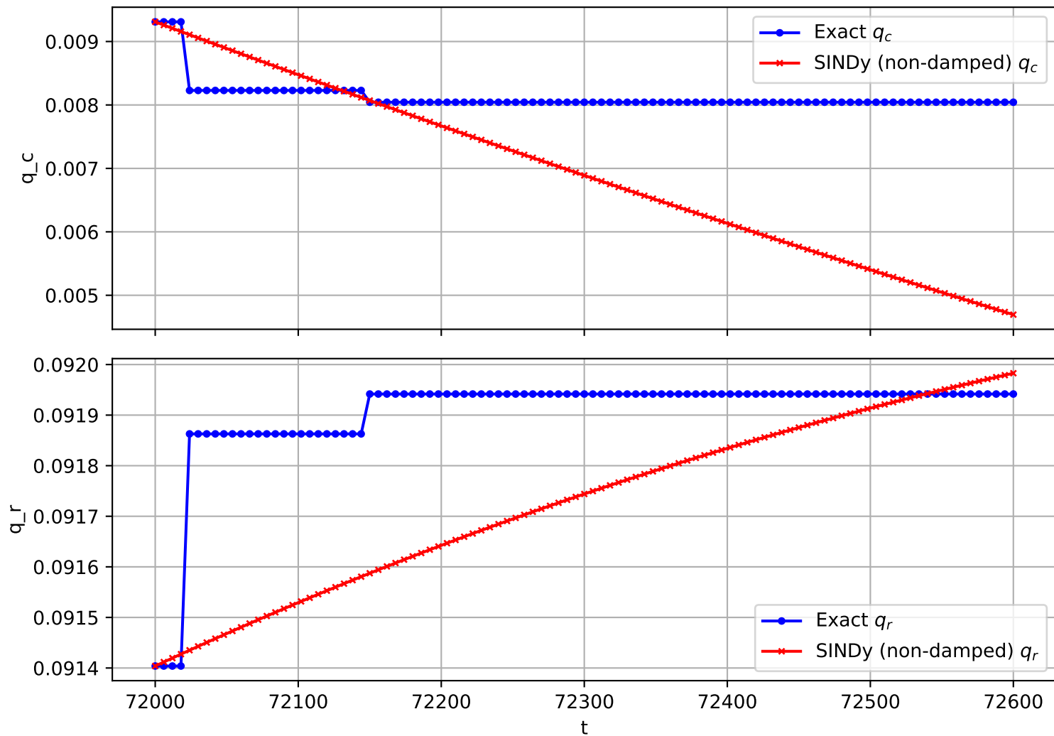
Trajectory 3030 (non-damped)
