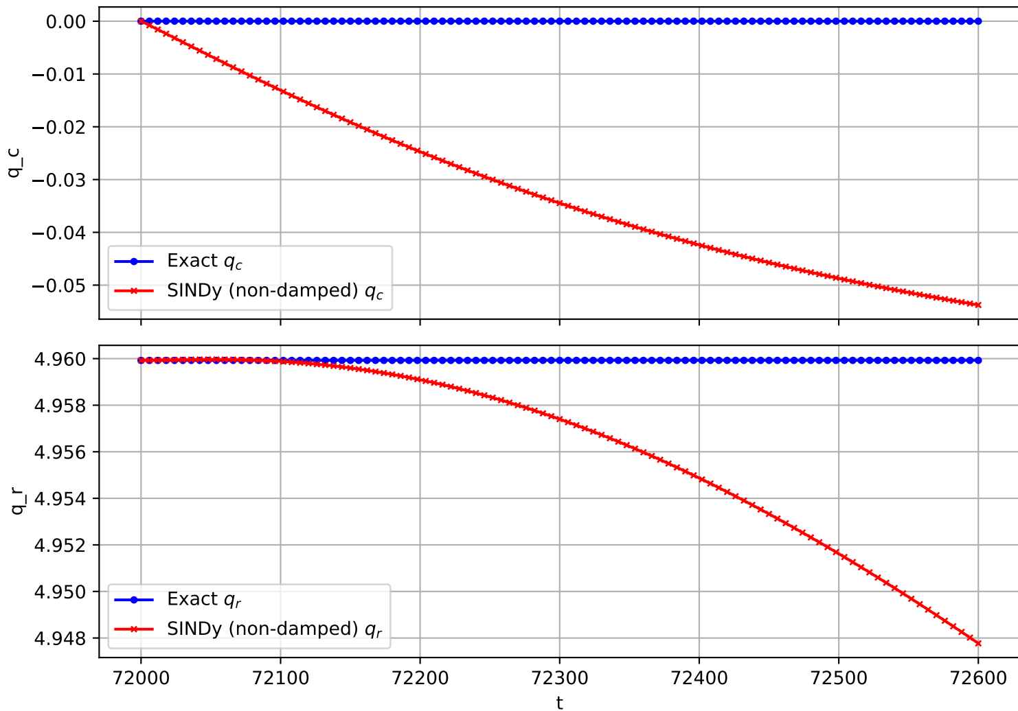
Trajectory 316 (non-damped)
