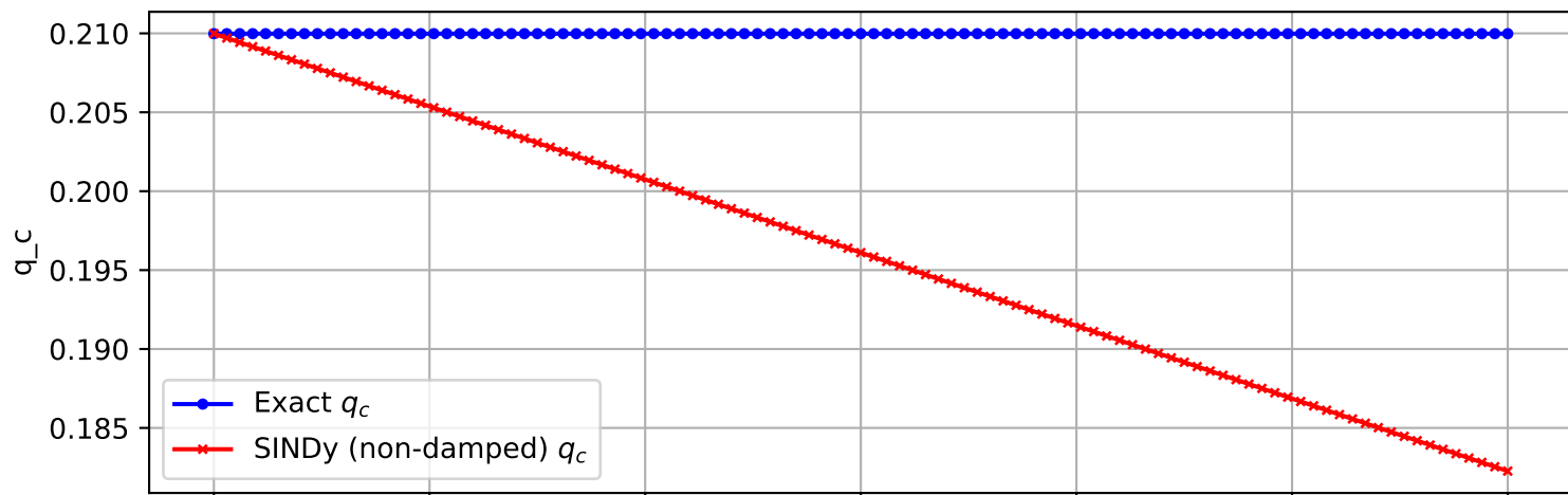
Trajectory 33 (non-damped)
